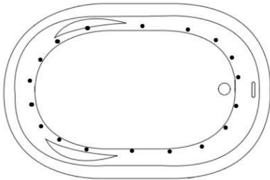
18 Jet Air Tub (1) 115v 20AMP GFCI Circuit 1 Motor Location
