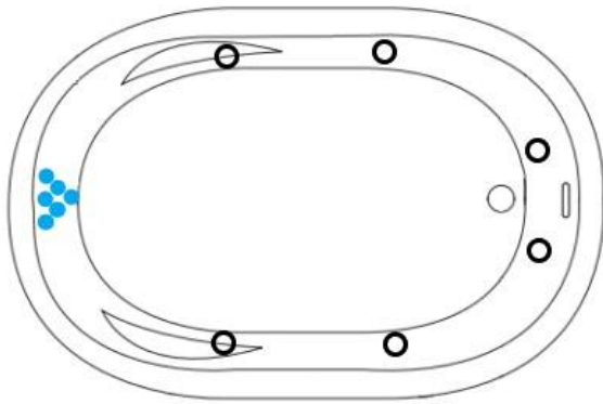
12 Jet Whirlpool (2) 115v 20AMP GFCI Circuits 1 Motor Location
